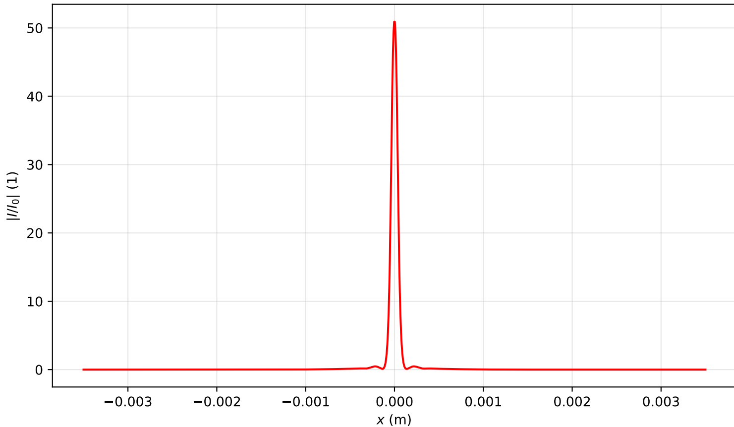
Intensity profile I(x, y = 0, z = 1.194)/I_0 , P_{in}=2.0P_{cr} , artificial time
